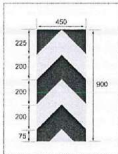
Two way Hazard Marker, Sign W70
