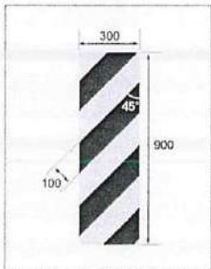
Object Hazard (Right), Sign W69
